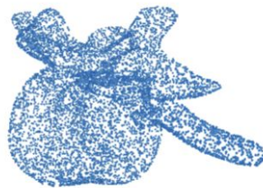
SSM-Net*
