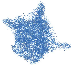
UBone3D (Ours)
